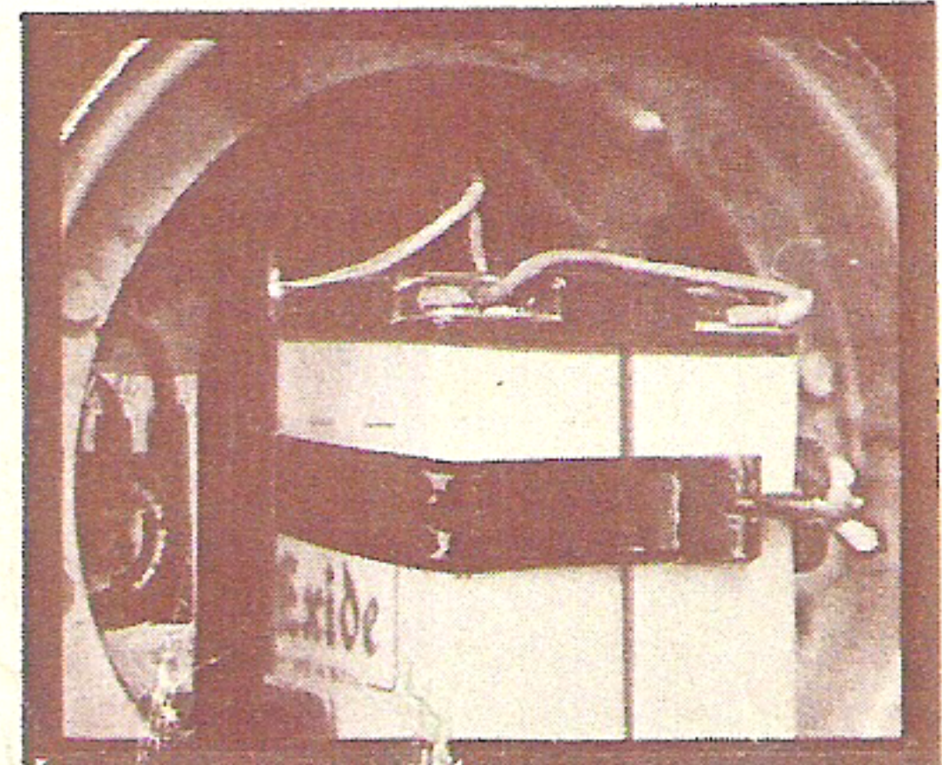
Vespa 160-180 Battery mounting
